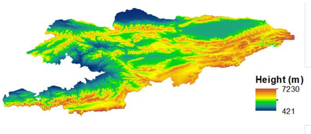
FIGURE 5. Shuttle Radar Terrain Mission Digital Elevation Model (STRM-DEM) at 30 m resolution
